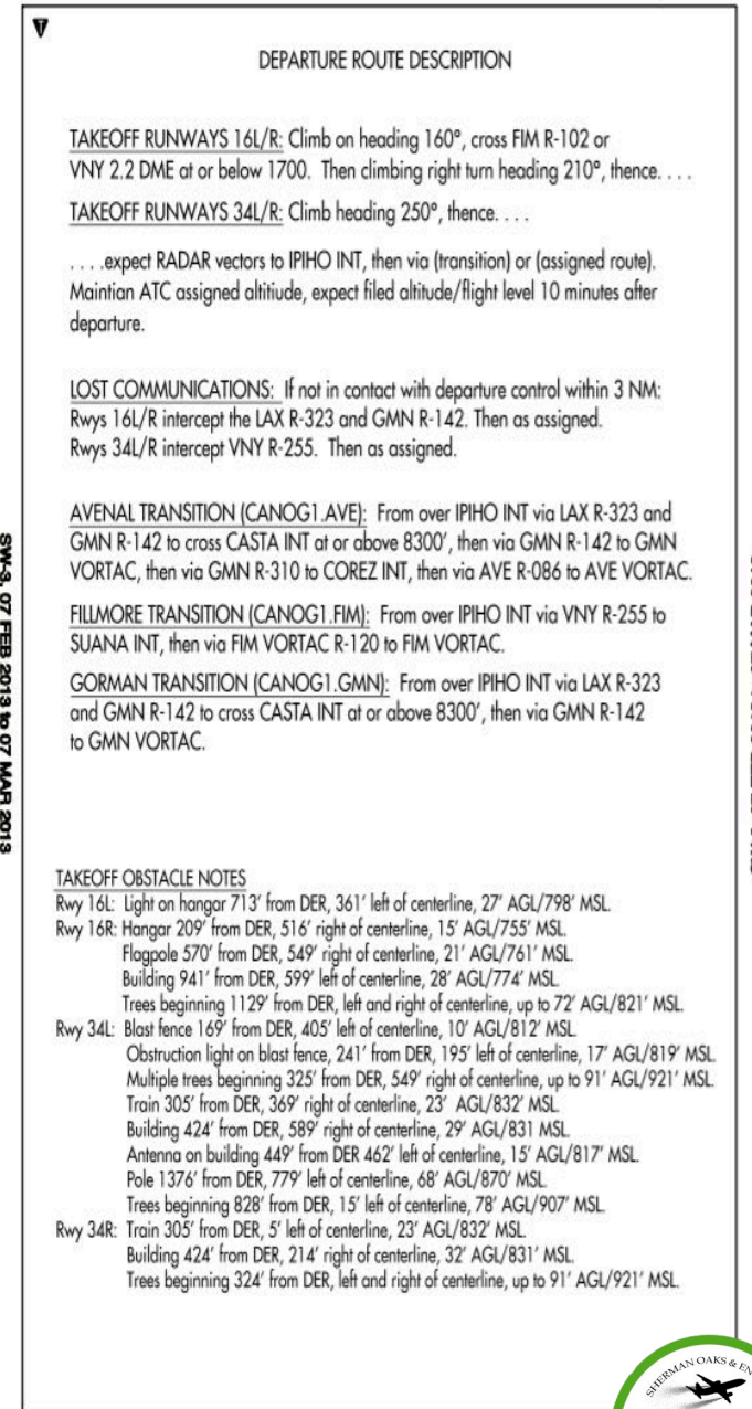
CANOGA ONE DEPARTURE (CANOG1.VNY) 12208
